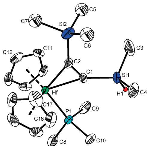
Figure 2. Molecular structure of compound 11 . Atoms with higher occupancy are shown for the disordered \text{SiMe}_3 group. Hydrogen atoms are omitted for clarity, except for H1. Thermal ellipsoids correspond to the 30% probability level. Selected bond lengths (Å) and angles (deg): Hf–C1 = 2.254(6), Hf–C2 = 2.196(7), C1–C2 = 1.296(9), C1–Si1 = 1.852(7), C2–Si2 = 1.863(8), C1–Hf–C2 = 33.8(2), C1–C2–Si2 = 141.4(6), C2–C1–Si1 = 130.0(6).
