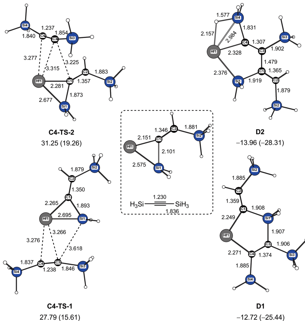
Scheme 9. BP86 Computed Bond Distances (Å), Gibbs Free Energies ( \Delta G , kcal/mol), and Enthalpies ( \Delta H , kcal/mol, in Parentheses) for the Insertion Reaction of the Second Molecule of the Alkyne Substrate to Intermediate C a
