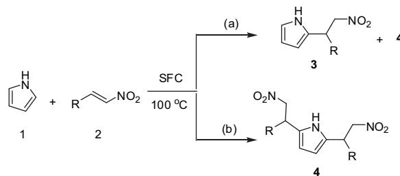
Scheme 1. Reaction of pyrrole with various \beta -nitrostyrenes: (a) 1 mmol of \beta -nitrostyrene ( 2 ) was used, at 100 °C. (b) 2.4 mmol of \beta -nitrostyrene ( 2 ) was used, at 100 °C.
