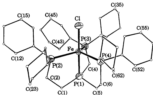
Figure 2. Molecular structure of the cation of [FeCl(PP 3 Cy)]BPh 4 . The hydrogen atoms are omitted for clarity.
