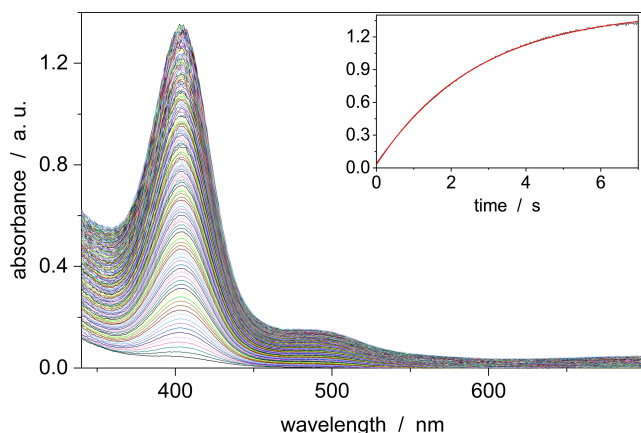
Figure 7. Time resolved stopped-flow UV-vis spectra of the formation of copper(I) bis( \mu -oxido) complex with ligand 12 in acetone ( C_{\text{complex}} = 0.50 \cdot 10^{-3} \text{ mol L}^{-1} , C_{\text{O}_2} = 5.7 \cdot 10^{-3} \text{ mol L}^{-1} , after mixing) at -93.0^{\circ}\text{C} . Inlay (time trace): Absorbance vs. time at 405 nm (black: experimental, red: exponential fit).
