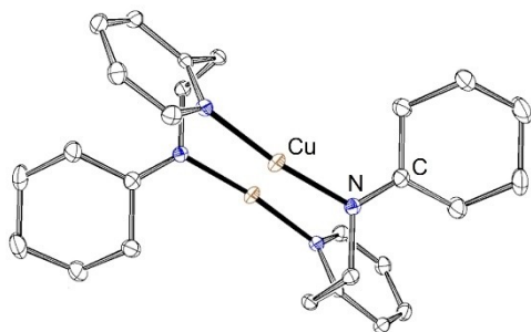
Figure 5. ORTEP plot of molecular structure of [Cu 2 (14) 2 ](OTf) 2 . Hydrogen atoms and counter ions are omitted for clarity. Anisotropic displacement ellipsoids set to 50% probability.
