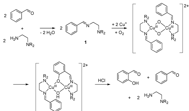
Scheme 1. Intramolecular hydroxylation of [\text{Cu}(1)]^+ complex ( R = \text{Et} ) with dioxygen. The hydroxylation proceeds via a copper bis( \mu -oxido) intermediate. [6]
