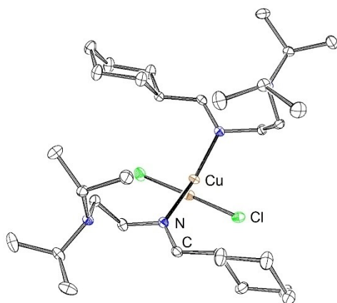
Figure 3. ORTEP plot of the molecular structure of [\text{Cu}(\mathbf{9})_2][\text{CuCl}_2] . Hydrogen atoms are omitted for clarity. Anisotropic displacement ellipsoids set to 50% probability.
