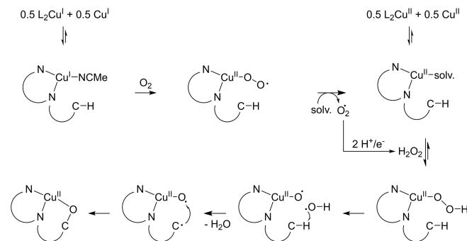
Scheme 2. Proposed mechanism for the intramolecular hydroxylation of sp^2 C–H bond. Redrawn from Trammell et al. [11]
