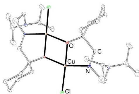
Figure 4. ORTEP plot of molecular structure of [\text{Cu}_2(\text{O}-\text{CyDiPED})_2\text{Cl}_2] . Hydrogen atoms are omitted for clarity. Anisotropic displacement ellipsoids set to 50% probability.
