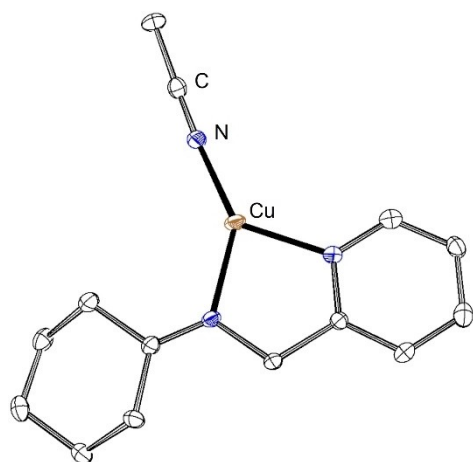
Figure 6. ORTEP plot of the molecular structure of the cation of [Cu(15)(MeCN)]OTf. Hydrogen atoms are omitted for clarity. Anisotropic displacement ellipsoids set to 50% probability.
