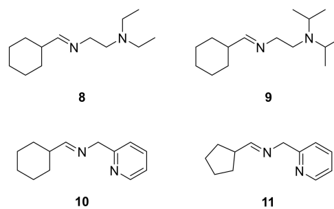
Scheme 4. Ligands CyDED ( 8 ), CyDiPED ( 9 ) and CyMPy ( 10 ), substrate: cyclohexane carboxaldehyde and ligand CypMPy ( 11 ), substrate: cyclopentane carboxaldehyde.
