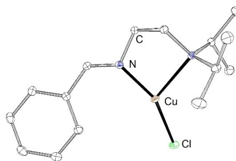
Figure 2. ORTEP plot of molecular structure of [Cu(2)]Cl. Hydrogen atoms are omitted for clarity. Anisotropic displacement ellipsoids set to 50% probability.
