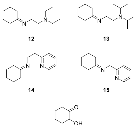
Scheme 6. Ligands CyonDED (12), CyonDiPED (13), CyonEPy (14), and CyonMPy (15), bottom: hydroxylated product 2-hydroxycyclohexanone.
