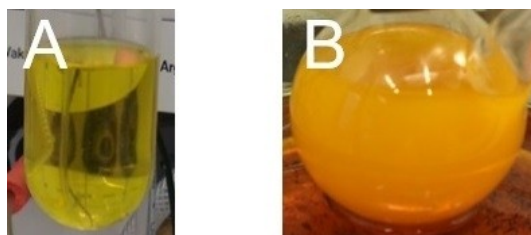
Figure 1. (A) The 1:1 [Cu:L] complex [Cu(1)]OTf in acetone and (B) the 1:2 [Cu:L_2] complex [Cu(1)_2]OTf in acetone.
