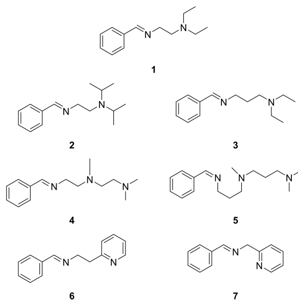
Scheme 3. Ligands used in this study: BDED ( 1 ), BDIPED ( 2 ), BDPD ( 3 ), BTED ( 4 ), BTPD ( 5 ), BEP ( 6 ) and BMP ( 7 ).
