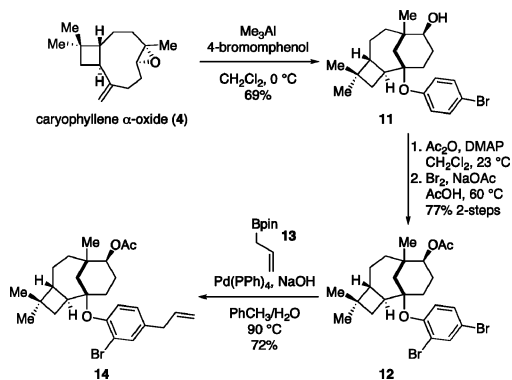
Scheme 2. Synthesis of Bromide 14
