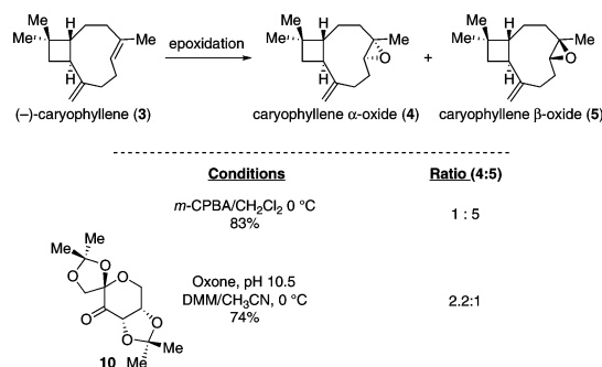
Figure 1. Diastereoselective epoxidation of (–)- \beta -caryophyllene.
