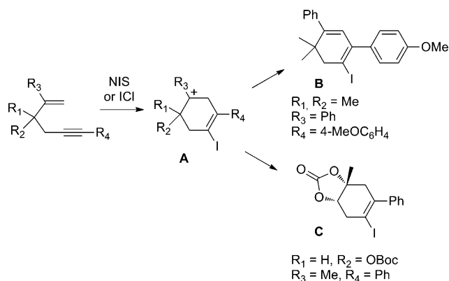
Scheme 1. Examples of Iodocyclization Reactions
