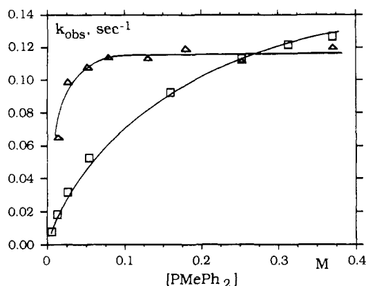
Figure 2. Plot of k_{\text{obs}} vs \text{PMePh}_2 concentration for the reactions of (\text{C}_5\text{Me}_5)\text{Rh}(\text{CO})(\text{X})(\text{Me}) : ( \Delta ) \text{X} = \text{MeCO}_2 ( 1d ); ( \square ) \text{X} = \text{CF}_3\text{CO}_2 ( 1e ).
