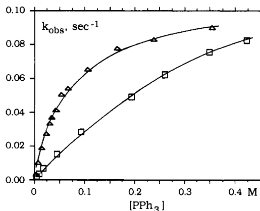
Figure 1. Plot of k_{obs} vs PPh_3 concentration for the reactions of (C_5Me_5)Rh(CO)(X)(Me) : ( \Delta ) X = MeCO_2 (1d); ( \square ) X = CF_3CO_2 (1e).
