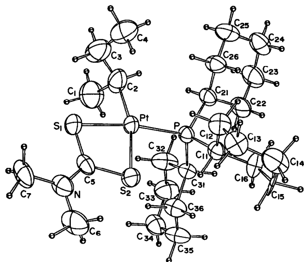
Fig. 1. ORTEP drawing of (\text{Me}_2\text{NCS}_2)\text{Pt}(\text{PCy}_3)(\text{sec-butyl}) .
