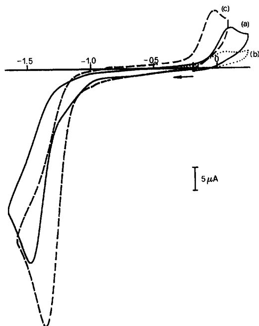
Fig. 1. Cyclic voltammograms for cis -[Cl 2 Pd(PPh 3 ) 2 ][CN(C 6 H 4 OMe- p )CH 2 CH 2 NH]] 1.0 mM, in 0.2 M[Bu 4 N][BF 4 ]/NCMe, at a Pt electrode ( \nu = 100 \text{ mV s}^{-1} ). (a) Complex alone (solid line). (b) In the presence of PhI (25 equiv.) (dotted line). (c) In the presence of [Et 4 N]Cl (10 equiv.) (dashed line).
