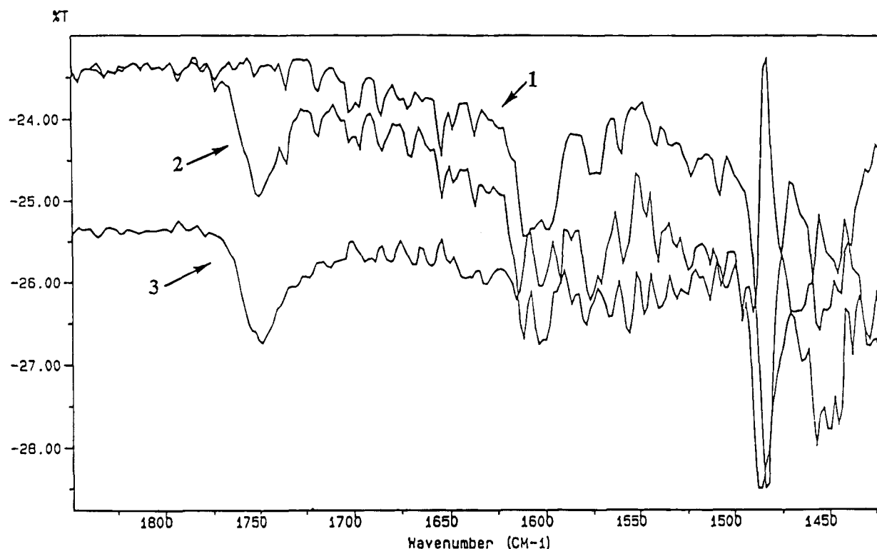
Figure 2. Low-temperature ( -75\text{ }^{\circ}\text{C} ) solution FT-IR spectra of [\text{Cu}(\text{CPY2-O}^-)(\text{Cl})\cdot 2\text{H}_2\text{O}] ( 9 ) (spectrum 1) and [\text{Cu}(\text{CPY2-O}^-)(m\text{-ClC}_6\text{H}_4\text{C}(\text{O})\text{OO}^-)] ( 3 ) (spectrum 2) and the difference of spectra 1 and 2 (spectrum 3) in \text{CH}_2\text{Cl}_2 ( \text{CH}_2\text{Cl}_2 as the background). Note the appearance of a peak at 1748\text{ cm}^{-1} for 3 .
