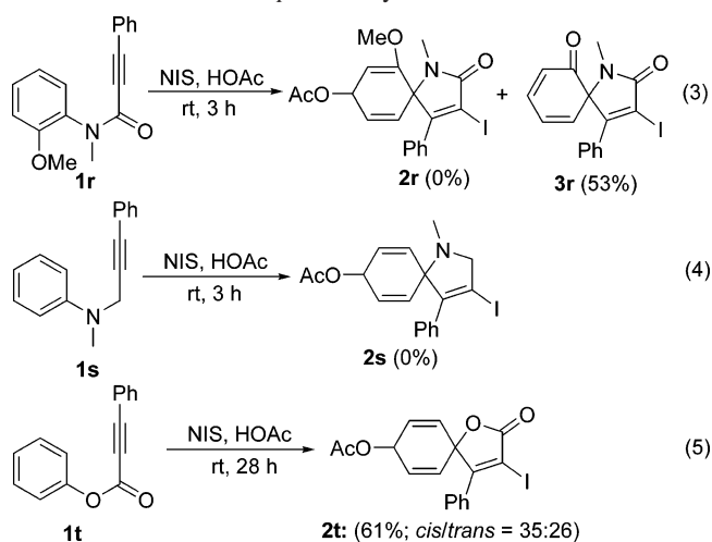
Scheme 1. ipso -Iodocyclization Reaction
