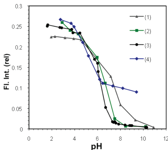
Figure 2. Fluorescence response to pH for compounds 1–4 measured using 0.37 \mu M solutions in 15% EtOH/H 2 O (v/v). Excitation wavelength was 550–560 nm. Fluorescence intensities are relative to a 0.37 \mu M solution of rhodamine B in H 2 O.
