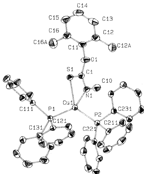
Figure 2. ORTEP view of [\text{Cu}\{\text{SC}(\text{OC}_6\text{H}_3-2,6-\text{Me}_2)=\text{NMe}\}(\text{PPh}_3)_2] ( 4 ).
