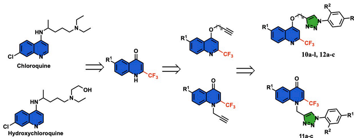
Fig. 2. Designing of quinoline-triazole conjugates.
