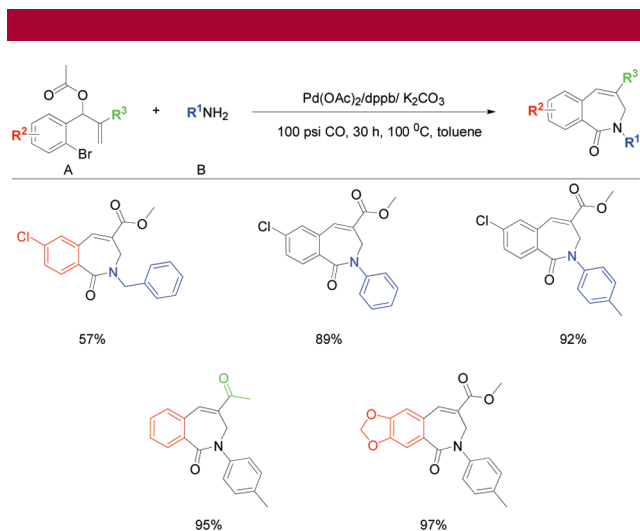
Figure 2. Substrates scope of the palladium-catalyzed amination and intramolecular cyclocarbonylation reactions of different Baylis–Hillman acetates. Reaction conditions: A (1 mmol), B (3 mmol), \text{K}_2\text{CO}_3 (2 mmol), \text{Pd(OAc)}_2 (0.05 mmol), dppb (0.1 mmol), toluene (5 mL).
