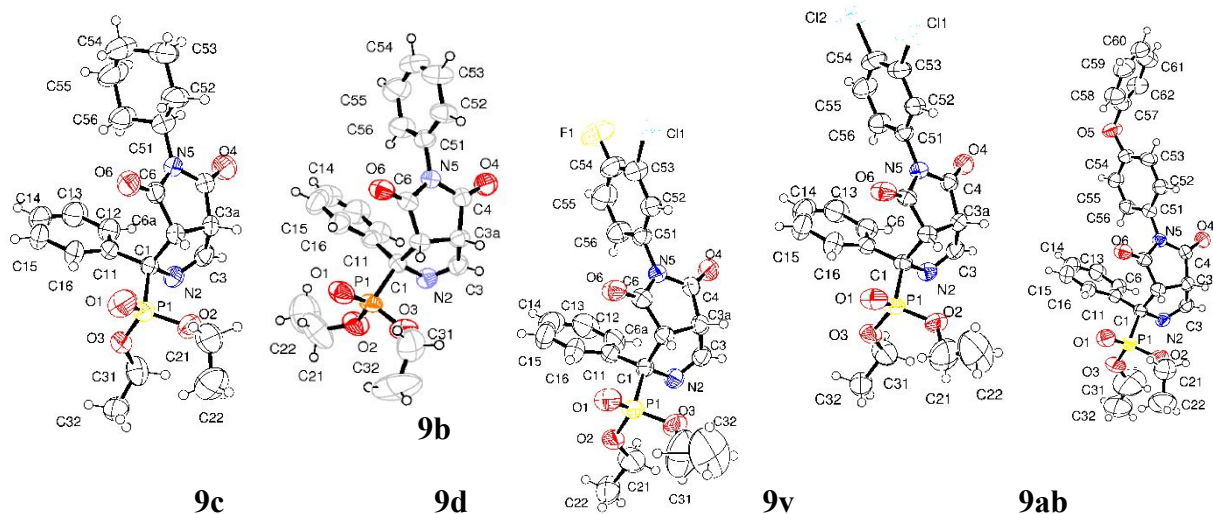
Figure 3. X-Ray structures of 9b , 9c , 9d , 9v and 9ab .
