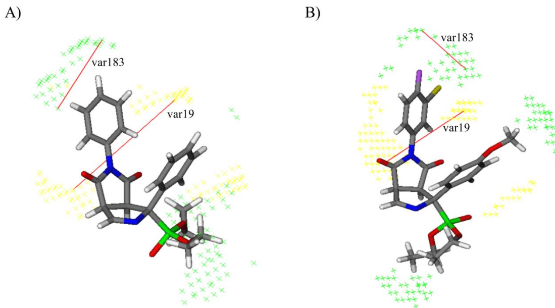
Figure 5. Representation of positive (in red) interactions of 9c (A) and 13d (B) in I 2 -IR
