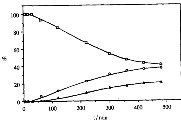
Fig. 2. Progress of the catalytic hydrogenation of diphenylacetylene promoted by complex 1 (reaction conditions: T = 80^\circ\text{C} , 8 ml of toluene, P(\text{H}_2) = 1 atm, [\textbf{1}]_{t=0} = 0.146 \times 10^{-2} M, [\text{Ph}_2\text{C}_2]_{t=0} = 0.146 M).
