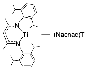
Scheme 1. Nacnac Ligand Structure
