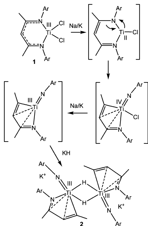
Scheme 2. Proposed Mechanism of Formation of 2
