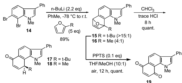
Scheme 2. Regioselectivity of 6,7-indolyne cycloadducts.
