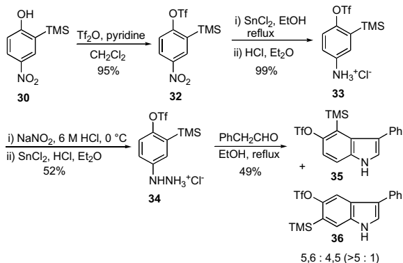
Scheme 7. Fischer indole synthesis of 4,5- and 5,6- o -trimethylsilyl triflate indolyne precursors.
