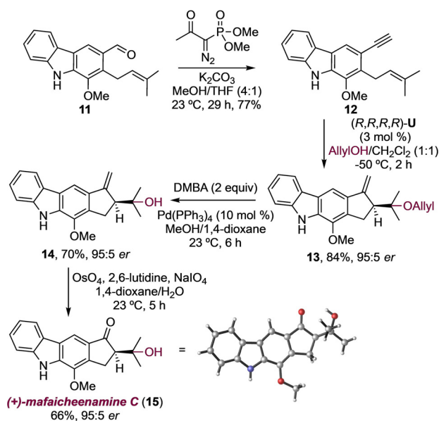
Scheme 4. Total synthesis of (+)-mafaicheenamine C. DMBA = dimethylbarbituric acid.
