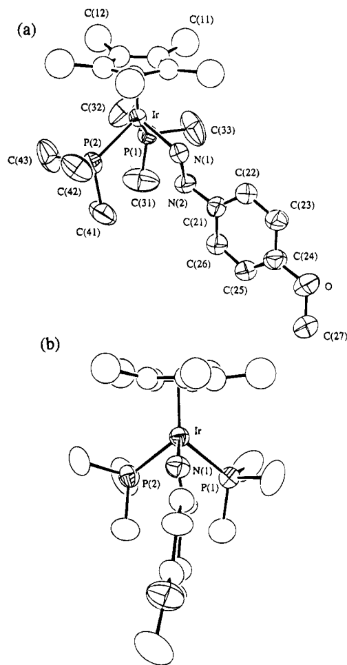
Figure 2. Molecular structure of the complex cation of 4. 50%-probability displacement ellipsoids for the non-hydrogen atoms are depicted. For clarity of presentation, only the major orientation of the disordered Cp* group is depicted. (b) View down the pseudo mirror plane that contains the aryldiazenido ligand.
