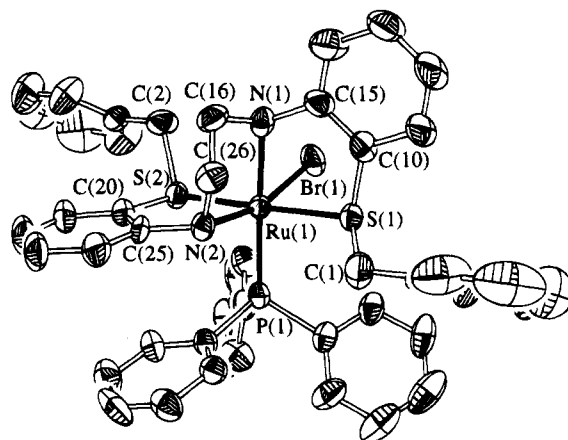
Figure 3. Molecular structure of [\text{Ru}(\text{Br})(\text{PPh}_3)(\text{'PhCH}_2)_2\text{S}_2\text{N}_2\text{H}_2)]\text{-Br} ( 9 ) (H atoms omitted).
