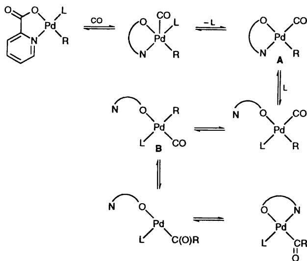
Scheme 4 Proposed carbonylation mechanism for the complexes [\text{PdMe}(\text{pyca})(\text{L})]
