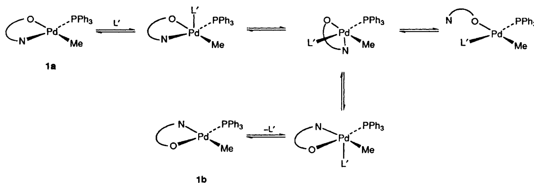
Scheme 2 Possible exchange reactions occurring in the presence of excess [\text{}^2\text{H}_5]\text{pyridine} ; \text{N} \rightarrow \text{O} = \text{pyca}
