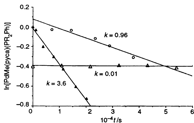
Fig. 1 Plots of carbonylation rates for the complexes [\text{PdMe}(\text{pyca})(\text{PPh}_3)] (▲), [\text{PdMe}(\text{pyca})(\text{PMePh}_2)] (○) and [\text{PdMe}(\text{pyca})(\text{PMe}_2\text{Ph})] (△)
