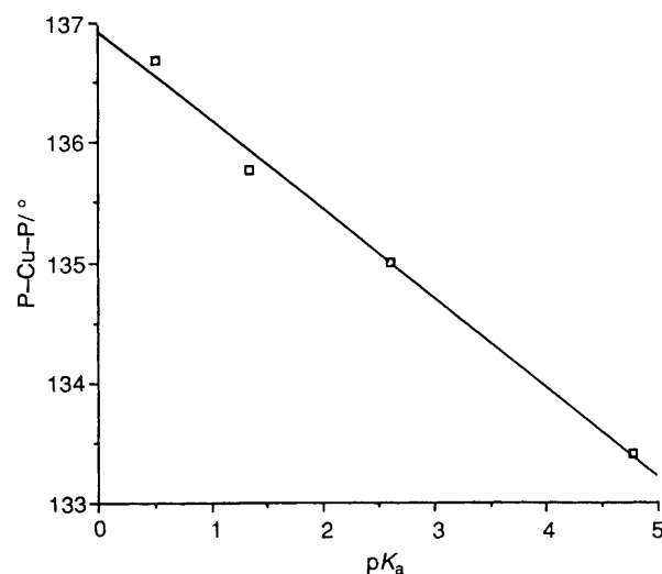
Fig. 3 Plot of the P-Cu-P angle of [\text{Cu}(\text{PPh}_3)_2(\text{O}_2\text{CCH}_3-n\text{F}_n)] complexes, n = 0-3 , as a function of \text{p}K_a
