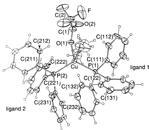
Fig. 2 Molecular structure of [\text{Cu}(\text{PPh}_3)_2(\text{O}_2\text{CCF}_3)(\text{EtOH})]
