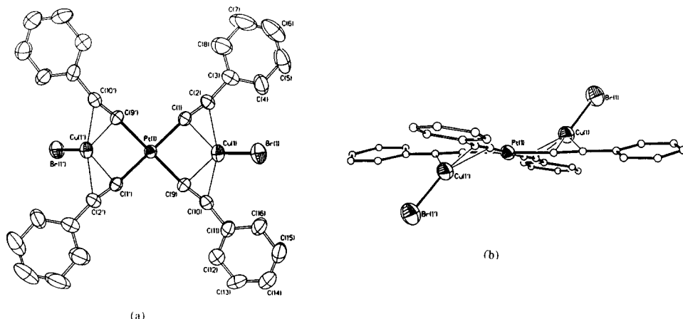
Fig. 1. (a) Drawing of the anion [\text{Pt}(\text{C}\equiv\text{CPh})_4(\text{CuBr})_2]^{2-} in complex 4 showing the atom-labelling scheme; (b) perspective showing the displacement of the CuBr groups out of the platinum coordination plane.
