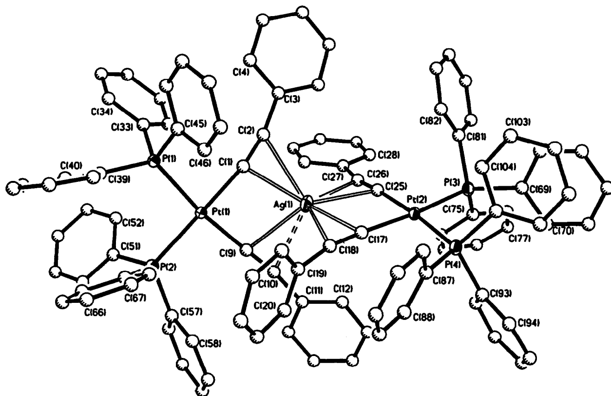
Fig. 1. View of the structure of the cation [\text{Pt}_2\text{Ag}(\text{C}\equiv\text{CPh})_4(\text{PPh}_3)_4]^+ in complex 1 with the atomic numbering scheme.
