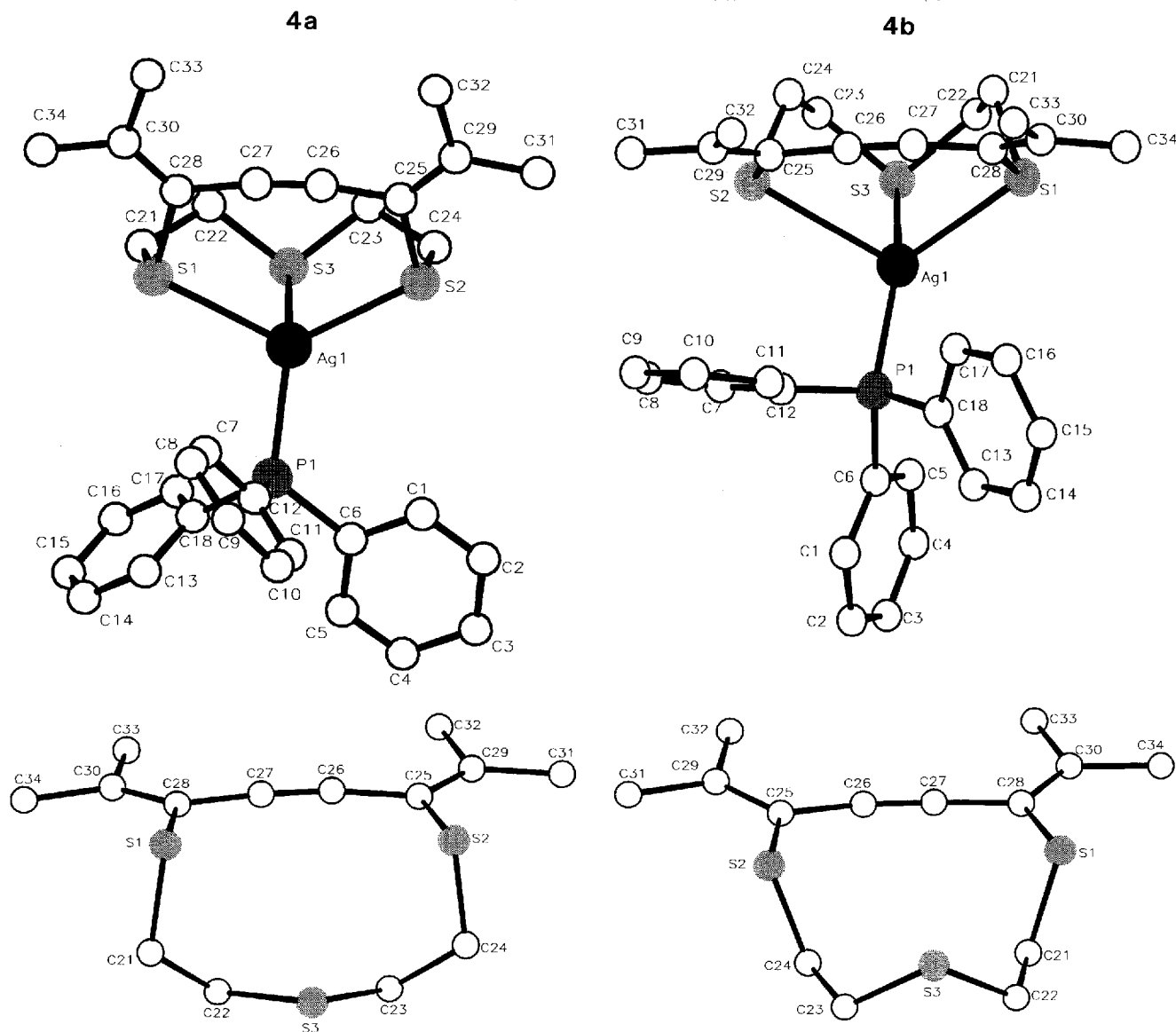
Figure 2. Molecular structures of 4a and 4b (top) and the respective macrocyclic ligand in 4a or 4b (bottom, Ag + and PPh 3 are omitted) in the crystal; selected bond lengths [Å] and bond angles [°] of 4a : Ag1–S1 2.752(3), Ag1–S2 2.643(3), Ag1–S3 2.572(4), Ag1–P1 2.410(3); S1–Ag1–S2 123.3(1), S1–Ag1–S3 83.5(1), S1–Ag1–P1 107.6(1), C26–C25–C29 125.5(8), C25–C26–C27 168.6(11), C24–S2–C25 102.2(5), C22–S3–C23 102.7(4), S2–C25–C26 112.5(7); 4b : Ag1–S1 2.750(2), Ag1–S3 2.500(2), Ag1–P1 2.387(2); S1–Ag1–S3 83.7(1), S1–Ag1–P1 119.9(1), S3–Ag1–P1 151.0(1), C26–C25–C29 124.8(5), C25–C26–C27 170.8(6), C24–S2–C25 101.6(3), C22–S3–C23 103.9(4), S2–C25–C26 113.0(5)
