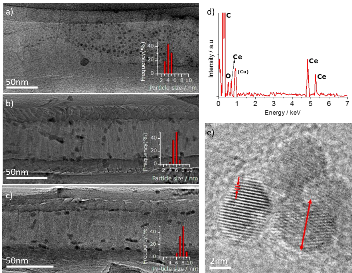
Figure 3. HRTEM analysis of \text{CeO}_2 nanoparticles encapsulated inside GNF ( \text{CeO}_2@\text{GNF} ). HRTEM images of \text{CeO}_2@\text{GNF} -1, -2 and -3 (a-c) and corresponding size distribution histograms of \text{CeO}_2 nanoparticles (inset). The EDX spectrum of \text{CeO}_2@\text{GNF} -3 (d) confirms the elemental composition and stoichiometry of Ce and O in \text{CeO}_2 (Ce:O is 0.5:1.0). HRTEM images of the \text{CeO}_2 nanoparticles encapsulated inside GNF (nanoparticle diameter indicated by the double-headed red arrow) showing d -spacing of 0.32 nm (e).
