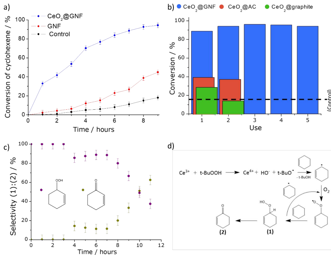
Figure 4. The conversion of cyclohexene obtained using \text{CeO}_2@\text{GNF} (here \text{CeO}_2@\text{GNF} -2) relative to control experiments as a function of time (a) and repeat use (b). The dotted horizontal line in (b) represents the conversion obtained in control experiments as reference. The change in selectivity for the products 2-cyclohexenyl hydroperoxide (1) and 2-cyclohexenone (2) with time (c), demonstrating the user-specificity of product selection using \text{CeO}_2@\text{GNF} . A proposed pathway for the oxidation of cyclohexene by ceria in \text{CeO}_2@\text{GNF} ; \text{Ce}^{3+} reacting with the peroxide reagent triggers a flux of radicals initiating a cycle of reactions with \text{O}_2 biradical leading to compound (1) which subsequently transforms to (2) (d).
