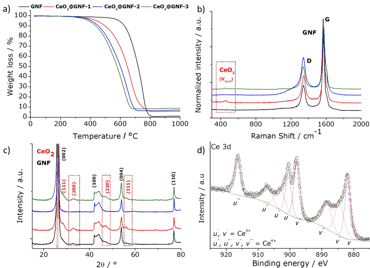
Figure 2. (a) TGA, (b) Raman spectroscopy, (c) PXRD and (d) XPS analysis of the CeO 2 @GNF nanocomposites. A decrease in the GNF combustion temperature and increase in the residual mass of CeO 2 obtained after GNF combustion observed in the thermograms (a) both correlate with the increasing amount of cerium complex used in the initial step. The Raman spectra (b) and PXRD patterns (c) of the CeO 2 @GNF nanocomposites both confirm the presence of both GNF and CeO 2 . Traces in (b) and (c) have been offset on the y-axis for visual clarity. The Raman spectra in (b) have been normalised to the intensity of the G-band. Annotated labels in (b) and (c) indicate Raman bands and diffraction planes corresponding to CeO 2 (red) and GNF (black). The fitted peak envelope for Ce 3d (d) in the XP spectrum confirms the presence of Ce 3+ which can act as an initiator in the reaction of cyclohexene and TBHP.
