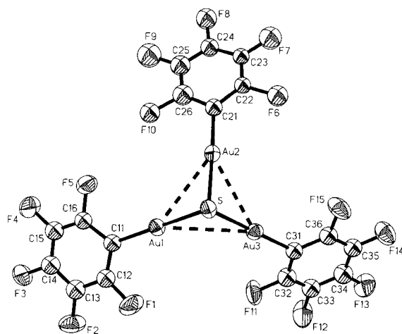
Figure 1. ORTEP plot of 7·Et 4 N·0.5MeC(O)Et with the labeling scheme. Selected bond lengths (Å) and angles (°): Au(1)–S, 2.301(4); Au(2)–S, 2.321(4); Au(3)–S, 2.319(4); Au(1)–Au(2), 3.277(9); Au(1)–Au(3), 3.477(9); Au(2)–Au(3), 3.184(9); Au(1)–C(11), 2.017(14); Au(2)–C(21), 2.019(14); Au(3)–C(31), 2.042(13). Au(1)–S–Au(2), 90.31(13); Au(1)–S–Au(3), 97.65(13); Au(2)–S–Au(3), 86.68(12); C(11)–Au(1)–S, 176.6(4); C(21)–Au(2)–S, 177.7(3); C(31)–Au(3)–S, 177.0(3).
