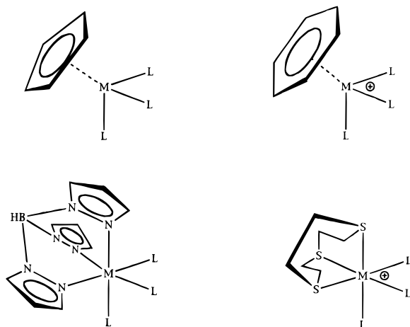
Chart 1. Coordination of 1,4,7-Trithiacyclononane [9]aneS 3 and Related Facially Tridentate Ligands
