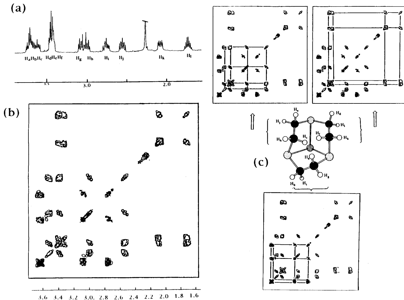
Figure 2. NMR spectroscopic analysis of [\text{Ru}(\text{CH}=\text{CHC}_6\text{H}_4\text{Me-4})\text{CO}](\text{PPh}_3)([\text{9}] \text{aneS}_3)\text{Cl} . (a) 1-D ^1\text{H} NMR spectrum in the region \delta 1.6–3.8 ppm ( \text{CH}_3 resonance augmented). (b) 2D- (^1\text{H}-^1\text{H}) COSY NMR spectrum in the region \delta 1.6–3.8 ppm. (c) Illustration of the three distinct ethylene coupling systems as a result of coordination of [\text{9}] \text{aneS}_3 to a chiral ruthenium centre.
