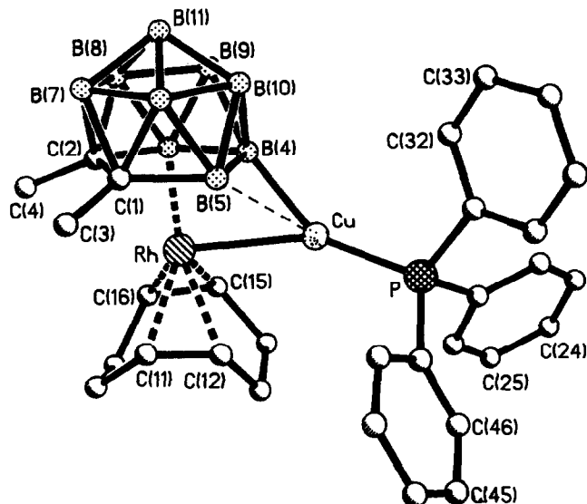
Fig. 1. Molecular structure of [\text{RhCu}(\text{PPh}_3)(\text{cod})(\eta^5\text{-7,8-C}_2\text{B}_9\text{H}_9\text{Me}_2)] (V) showing the crystallographic numbering scheme.
