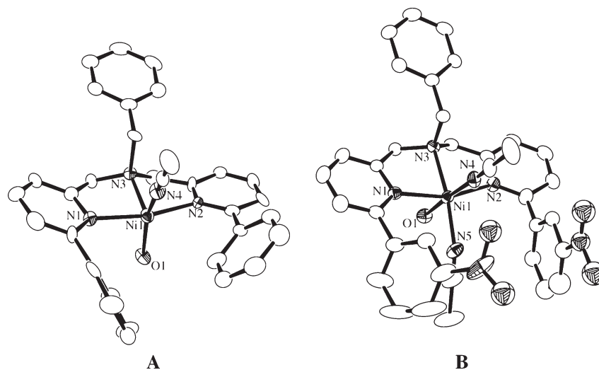
Figure 1. ORTEP drawings of the cationic parts of (A) [\text{Ni}^{\text{II}}(\text{L}^{\text{H}})(\text{CH}_3\text{CN})(\text{H}_2\text{O})](\text{ClO}_4)_2 ( 1 H ) and (B) [\text{Ni}^{\text{II}}(\text{L}^{\text{NO}_2})(\text{CH}_3\text{CN})_2(\text{H}_2\text{O})](\text{ClO}_4)_2 ( 1 NO_2 ) showing 50% probability thermal ellipsoids. The hydrogen atoms are omitted for clarity.
