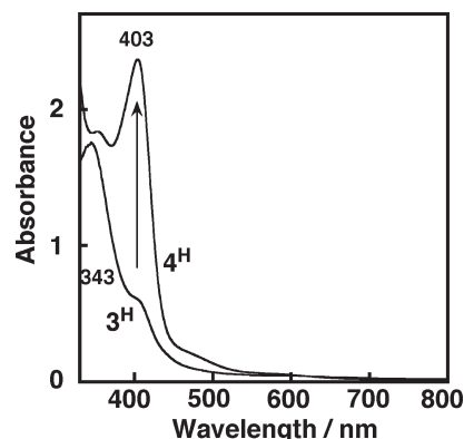
Figure 6. Spectral change for the conversion of 3^{\text{H}} to 4^{\text{H}} in acetone at room temperature.
