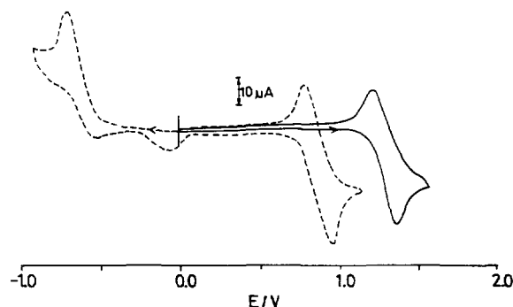
Fig. 3. Cyclic voltammograms of 1 (—) and 2 (---) in dichloromethane.
