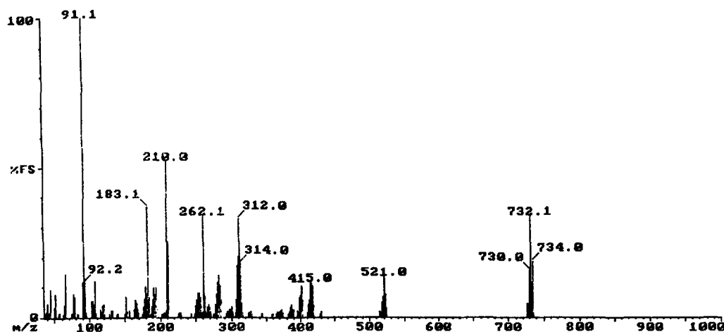
Fig. 6. Mass spectrum of 1.
