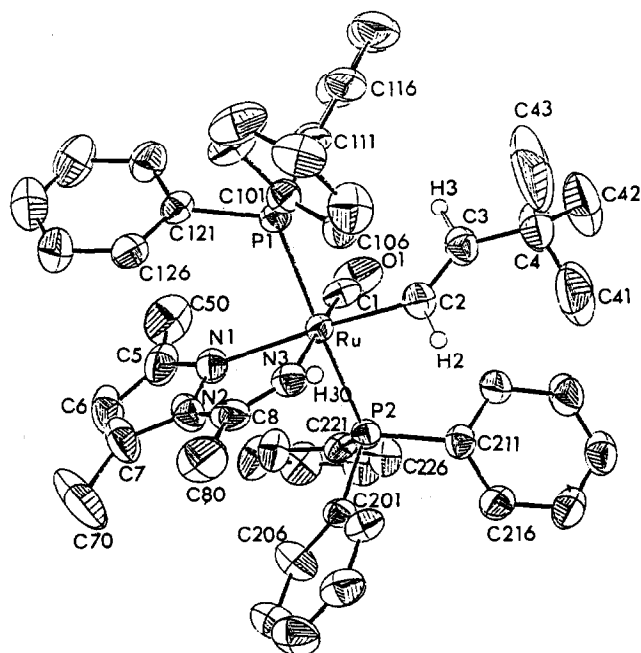
Fig. 1. ORTEP drawing of the structure of the cationic species [\text{Ru}(\text{CO})(\text{CH}=\text{CHCMe}_3)\{\text{NH}=\text{C}(\text{Me})(\text{Me}_2\text{pz})\}(\text{PPh}_3)_2]^+ (atom numbering as in Tables 1 and 3). Numbering of the carbon atoms of the phenyl rings and the hydrogen atoms of the phenyl, methyl and pyrazolyl groups omitted for clarity.
