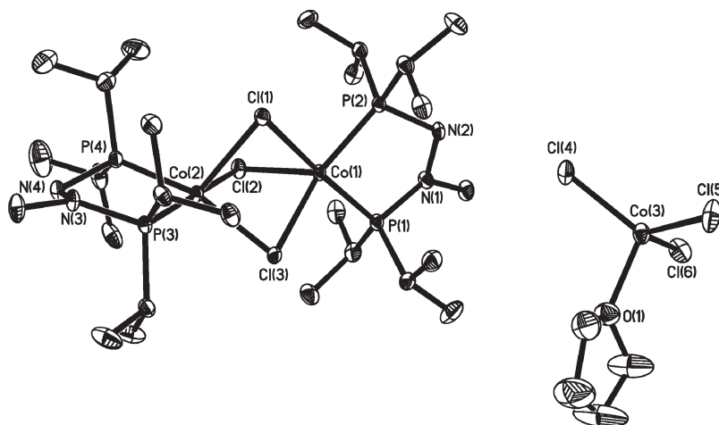
Figure 3. Molecular structure of [\text{Co}\{(\text{PiPr}_2\text{-NMe-NH-PiPr}_2)\text{-}\kappa^2\text{P,P'}\}_2(\mu\text{-Cl})_3][\text{CoCl}_3(\text{THF})] ( 11 ). Hydrogen atoms are omitted for clarity. Ellipsoids are drawn at 30% probability.
