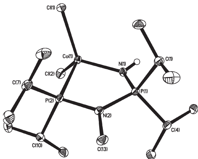
Figure 4. Molecular structure of [\text{CoCl}_2\{(\text{HN}=\text{PiPr}_2\text{-NMe-PiPr}_2)\text{-}\kappa^2\text{N,P}\}] ( 15 ). Hydrogen atoms other than H(1N) are omitted for clarity. Ellipsoids are drawn at 30% probability.
