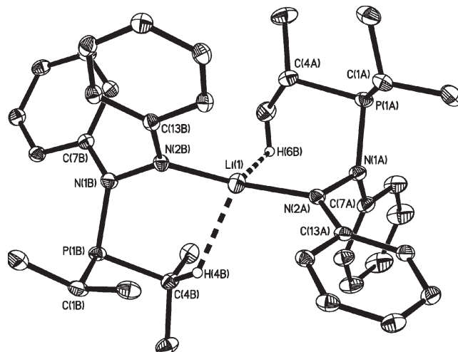
Figure 1. Molecular structure of [Li(DME) 3 ][Li{(NPh–NPh–P i Pr 2 )–κ N } 2 ] ( 5 ). Hydrogen atoms other than H4B and H6B and the Li(DME) 3 cation are omitted for clarity. Ellipsoids are drawn at 30% probability.
