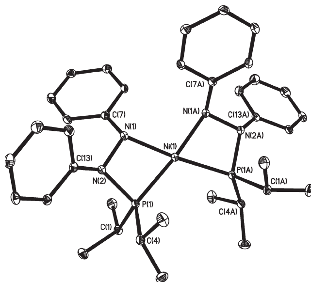
Figure 2. Molecular structure of [\text{Ni}\{(\text{NPh}-\text{NPh}-\text{P}(\text{iPr})_2)-\kappa^2\text{N},\text{P}\}_2] ( 6 ). Hydrogen atoms are omitted for clarity. Ellipsoids are drawn at 30% probability.
