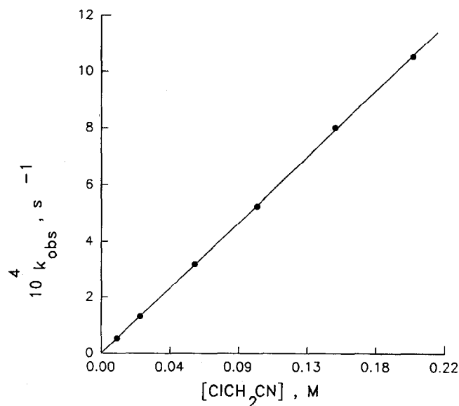
Fig. 1. Plot of k_{\text{obs}} vs. [ClCH_2CN] for the reaction of 1 with ClCH_2CN in acetonitrile at 25^\circ\text{C} .
