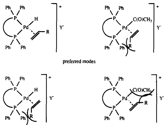
Fig. 4. Effect of the sterical hindrance on the stereochemistry of insertion of an alkene into a Pd-H bond and into a Pd-C(O)CH 3 bond.
