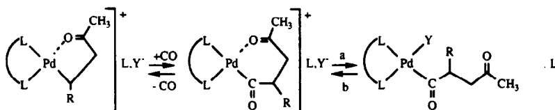
Fig. 2. Equilibria in the insertion of alkenes into the palladium-acyl bond. For \text{Y}^- = \text{Cl}^- , \text{L} = \text{solvent} : a > b . For \text{Y}^- = \text{SO}_3\text{CF}_3^- , \text{L} = \text{CH}_3\text{CN} : b > a .
