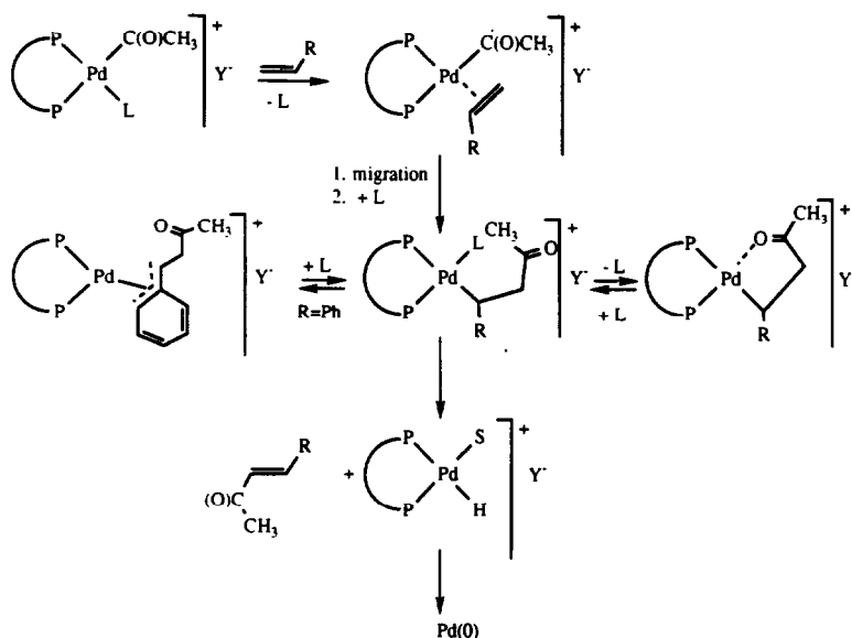
Scheme 1. Reaction scheme for the insertion of alkenes into the palladium-acyl bond ( Y^- = Cl^- or SO_3CF_3^- , in the latter case also CH_3CN present).
