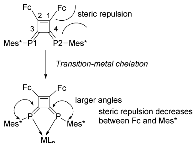
Chart 3. Schematic Chelation Effect on DPCB Complexes
