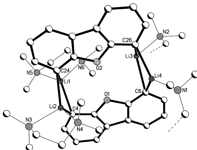
Figure 1. Stick and ball representation of 1. H atoms omitted for clarity. Only one conformation of the disordered tmeda ligand is shown. Selected bond lengths (Å) and angles (deg): Li(1)–N(5) 2.076(18), Li(1)–N(6) 2.154(17), Li(1)–C(4) 2.229(16), Li(1)–C(24) 2.280(17), Li(2)–N(3) 2.23(3), Li(2)–N(4) 2.21(2), Li(2)–C(4) 2.226(17), Li(2)–C(24) 2.235(17), Li(3)–N(2) 2.167(15), Li(3)–C(6) 2.333(14), Li(3)–C(26) 2.361(15), Li(4)–N(1) 2.022(16), Li(4)–C(6) 2.157(15), Li(4)–C(26) 2.231(14); N(5)–Li(1)–N(6) 91.4(7), C(4)–Li(1)–C(26) 108.9(7), N(4)–Li(2)–N(3) 84.7(8), C(4)–Li(2)–C(24) 110.7(7), N(2)–Li(3)–C(6) 112.0(6), N(2)–Li(3)–C(24) 106.8(6), C(6)–Li(3)–C(26) 107.2(6), N(1)–Li(4)–C(6) 124.7(7), N(1)–Li(4)–C(26) 115.2(6), C(6)–Li(4)–C(26) 118.8(7).
