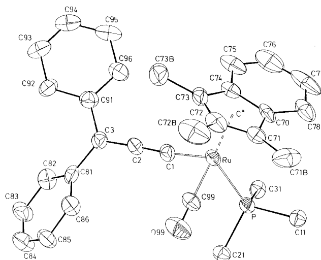
Figure 1. ORTEP drawing of 1. Selected bond distances (Å) and angles (deg): Ru–C1, 1.92(1); Ru–C99, 1.83(1); Ru–P, 2.349(3); Ru–C*, 1.93(1); C99–O99, 1.15(1); C1–C2, 1.26(1); C2–C3, 1.35(2); C3–C81, 1.47(2); C3–C91, 1.48(2); C99–Ru–C1, 92.1(5); C99–Ru–P, 86.8(4); C1–Ru–P, 92.5(3); O99–C99–Ru, 176.1(1); C2–C1–Ru, 172.1(1); C1–C2–C3, 176.1(1); C2–C3–C81, 120.1(1); C2–C3–C91, 120.1(1). C* = centroid of the indenyl ring.
