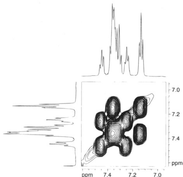
Figure 5. Section of the ambient temperature, phase-sensitive NOESY spectrum for 4b showing the exchange between the two different meta and two different para protons coming from the nonequivalent \text{PPh}_3 ligands.
