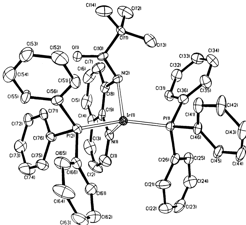
Figure 1. Diagram of the cation of [\text{Ir}(\text{H})_2(\text{PPh}_3)_2(\text{C}_9\text{H}_6\text{N}\{\text{HNCO}'\text{Bu}\})]\text{SbF}_6 ( 4b ). Thermal ellipsoids are at 50% probability. The hydrogen atoms have been omitted for clarity.
