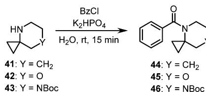
Scheme 4. Preparation of Starting Materials 44–46
