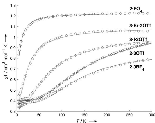
Figure 2. Plots of \chi_{\text{M}}T vs. T for compounds 2 and 3 at an applied field of 0.5\text{ T} . Solid lines represent the best fits obtained.
