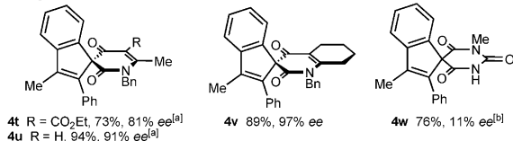
Scheme 4. Reactions were conducted with 0.20 or 0.30 mmol of 1 (see Supporting Information for details). Yields are of isolated products. Enantiomeric excesses were determined by HPLC analysis on a chiral stationary phase. [a] Dimethyl carbonate was used as the solvent. [b] The absolute stereochemistry of the major enantiomer of 4w is not known.
