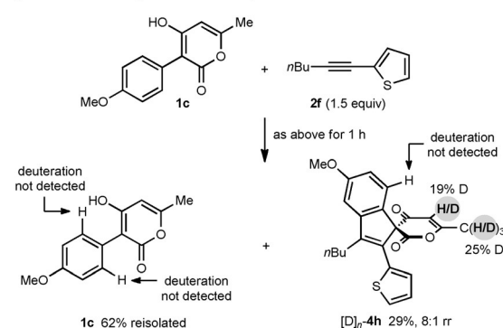
Scheme 5. Deuteration experiments.
