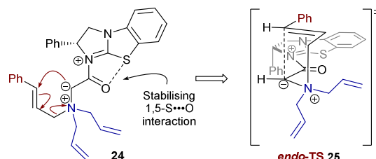
Figure 1: Stereochemical Rationale.
