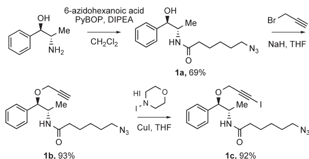
Scheme 1. Synthesis of Azido-Iodoalkyne Macrocycle Precursors
