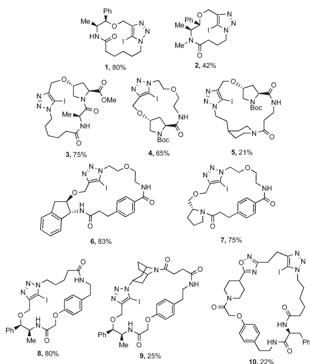
Figure 2. Substrate scope for the copper flow-mediated iodotriazole cyclization. Percentages correspond to isolated yields.
