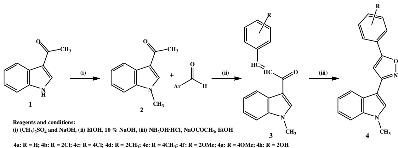
Scheme-I: Synthetic route of some novel N -methylated indole containing isoxazole moieties
