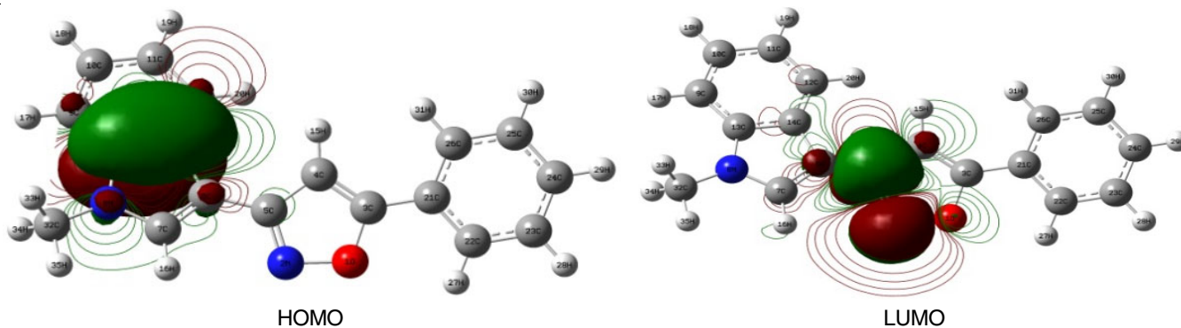
Fig. 2. HOMO and LUMO of 5-phenyl-3-(1-methylindol-3-yl)isoxazole ( 4a )
