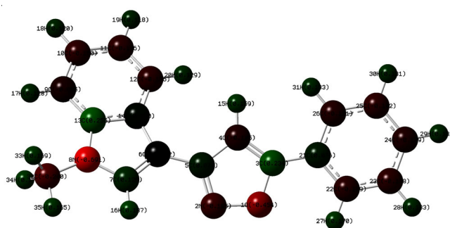
Fig. 3. Mulliken charge distribution of 5-phenyl-3-(1-methylindol-3-yl)-isoxazole ( 4a )
