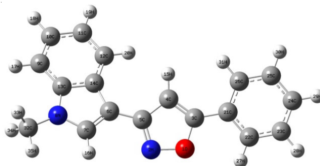
Fig. 1. Structure of 5-phenyl-3-(1-methylindol-3-yl)isoxazole ( 4a )
