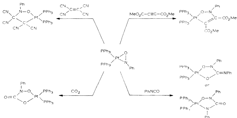
SCHEME 5
