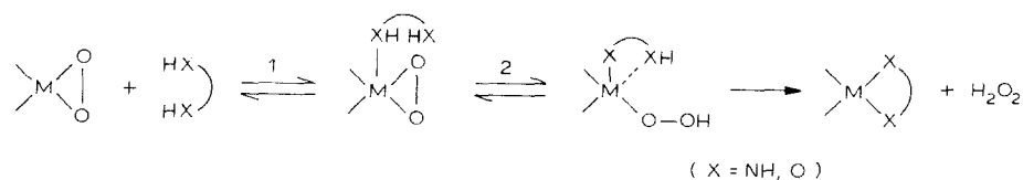
SCHEME 11
