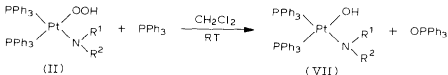
SCHEME 10
