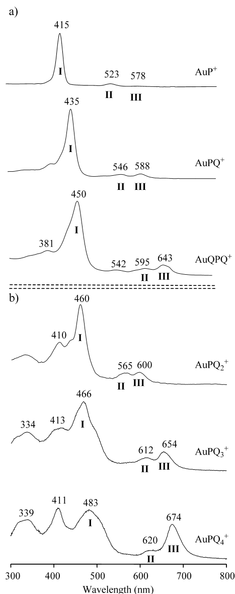
Figure 3. UV–visible spectra of (a) \text{Au}^{\text{III}}(\text{P})^+ , \text{Au}^{\text{III}}(\text{PQ})^+ , \text{Au}^{\text{III}}(\text{QPQ})^+ and (b) \text{Au}^{\text{III}}(\text{PQ}_2)^+ , \text{Au}^{\text{III}}(\text{PQ}_3)^+ , and \text{Au}^{\text{III}}(\text{PQ}_4)^+ in \text{CH}_2\text{Cl}_2 , 0.1 M TBAP.
