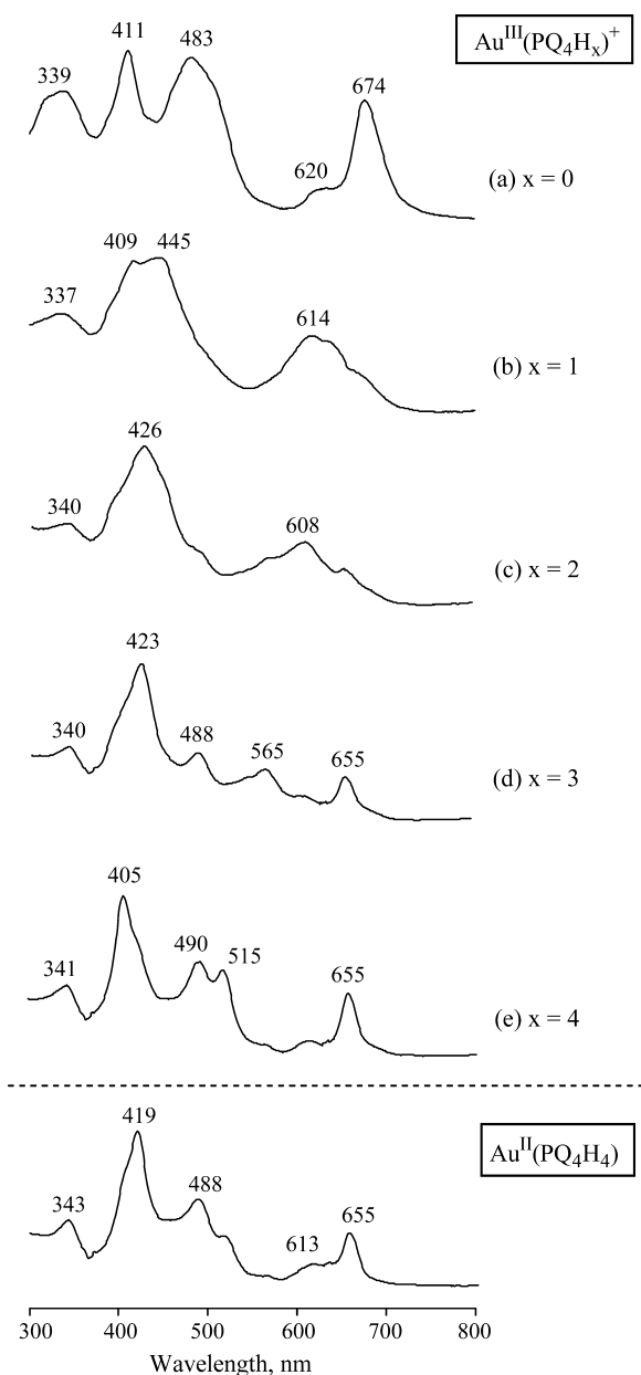
Figure 10. UV–visible spectra of \text{Au}^{\text{III}}(\text{PQ}_4)^+ and its stepwise reduction products in \text{CH}_2\text{Cl}_2 containing 0.1 M TBAP and 4.5 equiv of added TFA.
