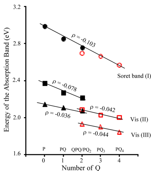
Figure 4. Plots of energy for the Soret and two visible bands of \text{Au}^{\text{III}}(\text{PQ}_n)^+ vs the number of Q groups on the macrocycle for P, \text{PQ} , and QPQ (black solid points) and \text{PQ}_2 , \text{PQ}_3 , and \text{PQ}_4 (red open points).
