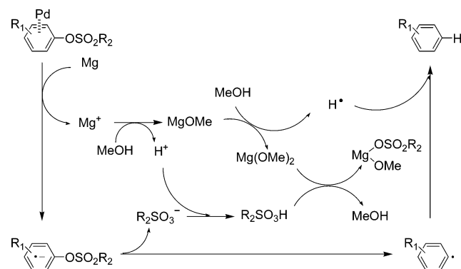
Scheme 1. Plausible Reaction Mechanism
